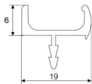
EH-AP053 ALUMINIUM HANDLE PROFILE
