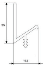
EH-AP065 ALUMINIUM HANDLE PROFILE
