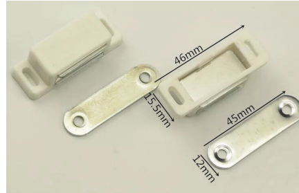
EH-MC110-MAGNETIC CATCH
