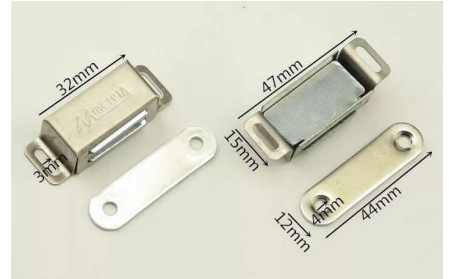
EH-SS110-MAGNETIC
