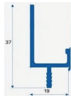
EH-AP061 ALUMINIUM HANDLE PROFILE
