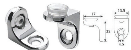
EH-GS3120-GLASS SHELF STUD
