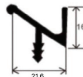
EH-AP062 ALUMINIUM HANDLE PROFILE
